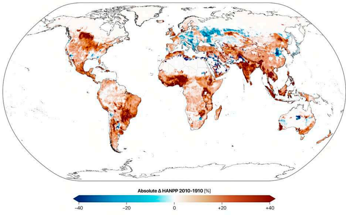
FIGURE 15 Change in Land Plant Energy Used by Humanity. Total change in the human appropriation of net primary production (HANPP) in 2010 compared to (minus) the HANPP in 1910, both expressed as a percentage of the potential (natural) NPP in 1910. A change from 10% to 30% HANPP would be indicated by a value of +20%. Shades of red indicate a HANPP increase and shades of blue indicate a decrease. Data from Kastner et al., 2022. 94 Key takeaway: The spatiotemporal patterns of HANPP changes were historically driven by land-use expansion and intensification. HANPP increased globally, except in parts of Eurasia where HANPP values were already very high and have recently shown a slight decrease.
