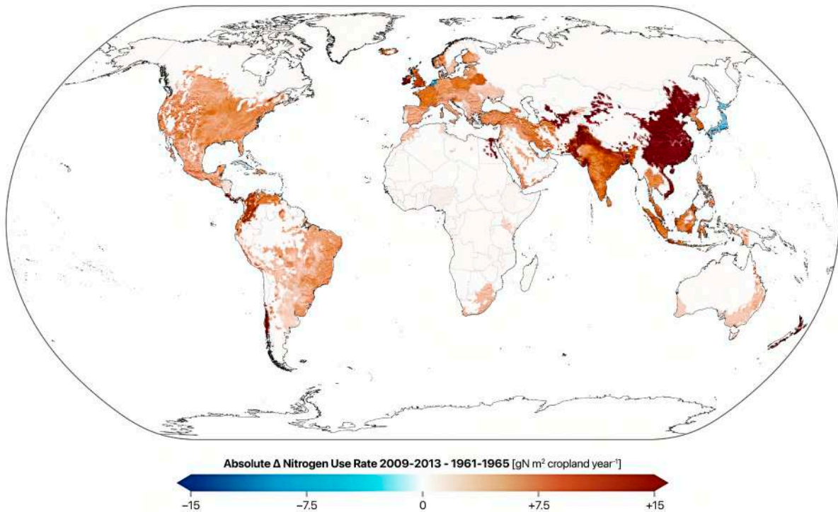
FIGURE 28 Global Map of Change in Nitrogen Use Rate for Agriculture Cycle. The total difference of nitrogen use rates (in \text{g N m}^{-2} \text{cropland year}^{-1} , e.g. grams of nitrogen per square meter cropland per year) calculated as the difference between the rates during the period 2009-2013 (last 5 years of data set) and the period 1961-1965 (first 5 years of data set). Data from Lu and Tian, 2017. 130 Key takeaway: The map highlights a global increase in nitrogen use, particularly in developing regions, raising concerns about environmental impacts and the need for sustainable agricultural practices.
